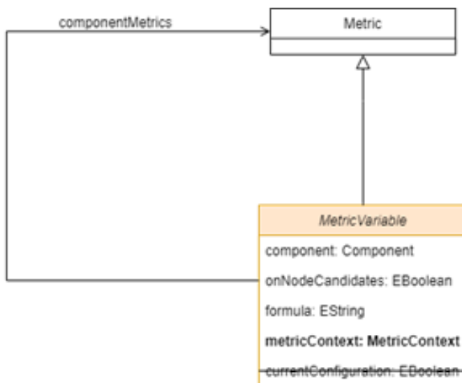
Figure 6 - The two CAMEL updates on MetricVariable class
